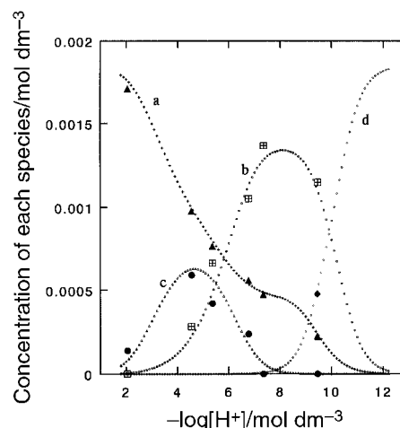
Fig. 3 Concentration of each boron species against pH in the equilibrated solution. Points refer to the experimental results, while the dotted lines are calculated. C_B = C_L = 0.00185 \text{ mol dm}^{-3} , I = 0.1 \text{ mol dm}^{-3} . a, \text{B(OH)}_3 ; b, 1:1 complex; c, 1:2 complex; d, \text{B(OH)}_4^- .
