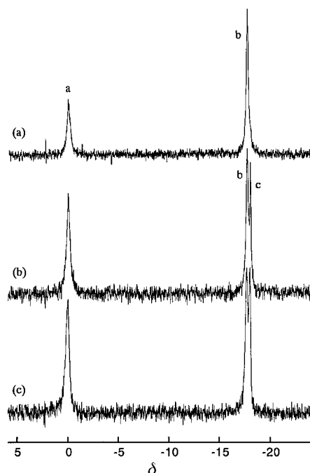
Fig. 4 ^{11}\text{B} NMR spectra for boric acid solutions with chromotropic acid at different reaction times. C_{\text{B}} = C_{\text{L}} = 0.00185 \text{ mol dm}^{-3} , I = 0.1 \text{ mol dm}^{-3} , pH 5.4. (a) for 0 h; (b) for 4 h; (c) for 17 h. a, Free boric acid; b, 1:1 complex; c, 1:2 complex.
